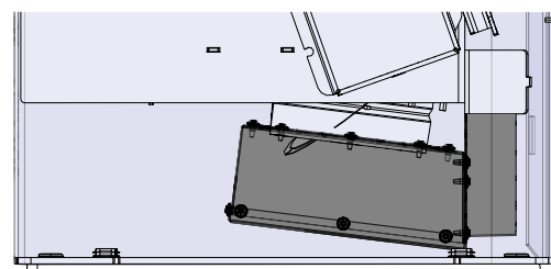
Abb. 11: Zuluftadapter montieren
